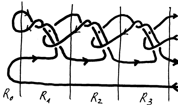
Figure 17: The wild knot R_0 R R R \dots
