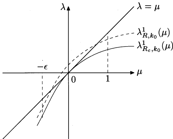
Figure 4: Graphical resolution of \lambda_{R, k_0}^1(\mu) = \mu
