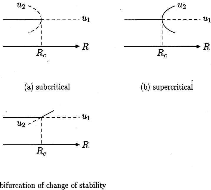
Figure 1: Different types of bifurcations
