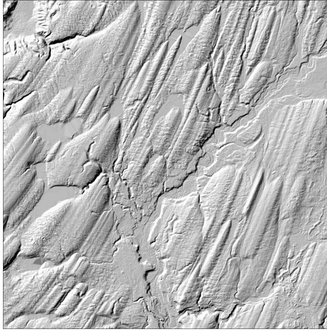
Figure 4. An aerial view of drumlinised topography in the environs of Seattle, Washington. The area shown is 6 \text{ km} \times 6 \text{ km} ; ice flow was from the upper right to the lower left, to the southwest. The image was calculated from the Puget Sound Lidar Consortium 6 foot digital elevation model, and is supplied courtesy of Ralph Haugerud.
