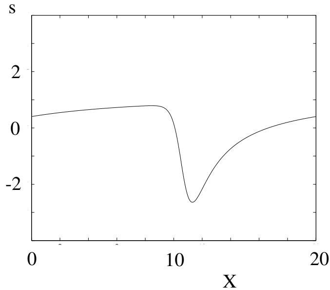
Figure 5. Solution of (26) starting from small amplitude random data, at T = 80 . The wave shown travels forward at a speed of approximately dX/dT = 0.73 .
