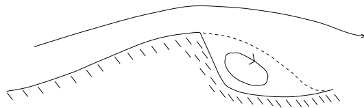
Figure 2. Separation in the lee of a transverse dune.
