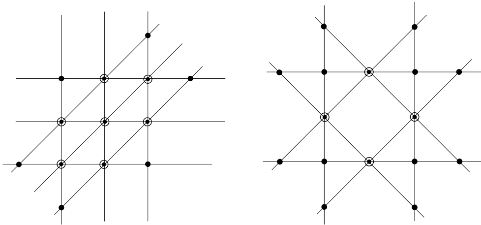
Figure 2. Two generalized natural lattices with 8 and 9 lines
