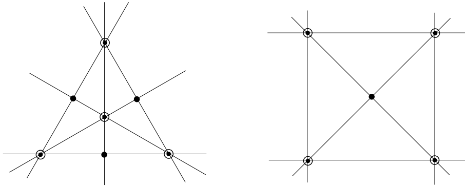
Figure 1. Two generalized natural lattices with 6 lines.
