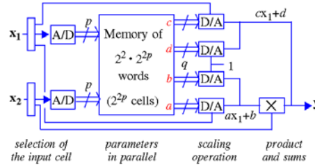
Figure 6: Memory-based parallel current-mode realization of a piecewise multilinear controller.
