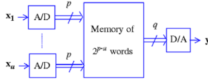
Figure 5: Look-up table realization for piecewise constant controller.
