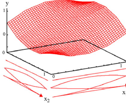
Figure 4: Example of a piecewise-biquadratic controller.
